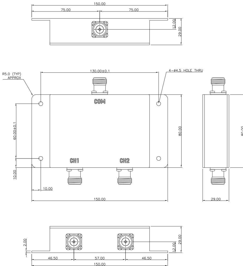
[ Mechanical 2D Drawing ]
