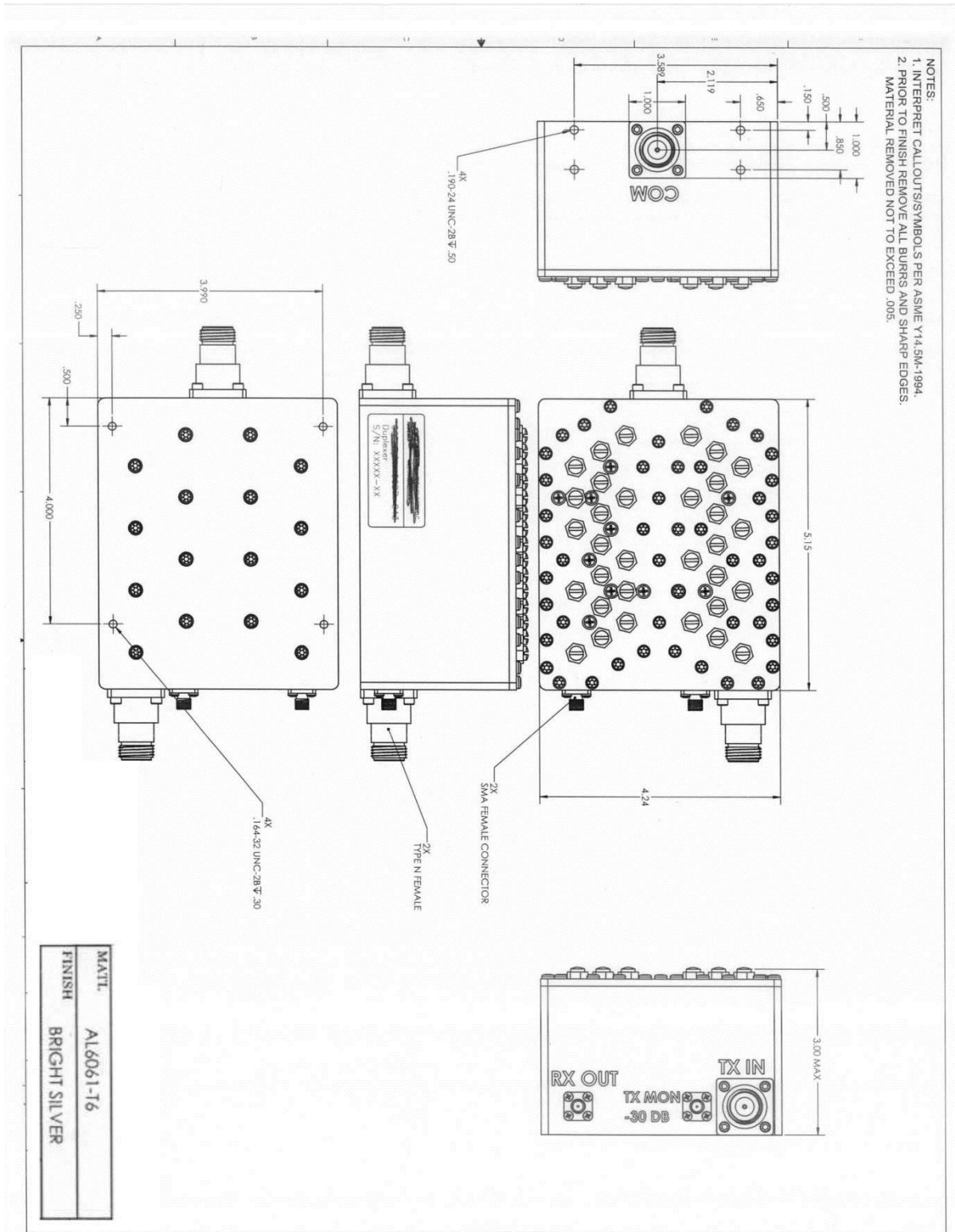
[ Mechanical 2D Drawing ]
