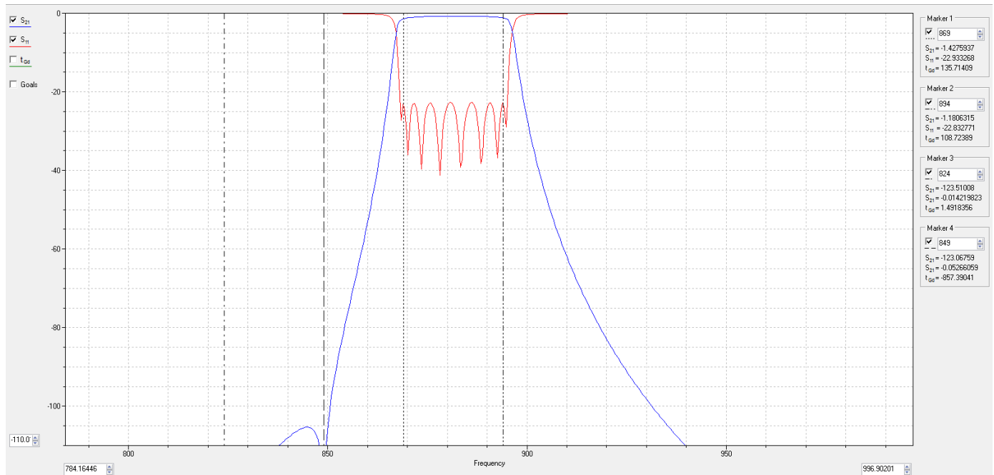
TX path
