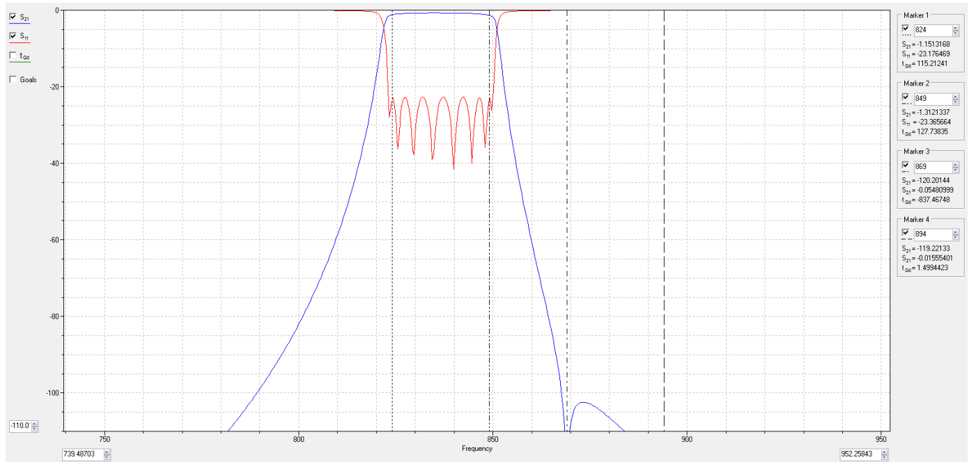
RX path
