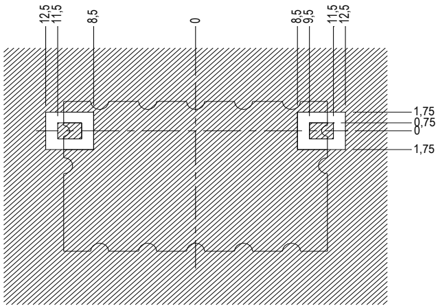
LAND PATTERN
