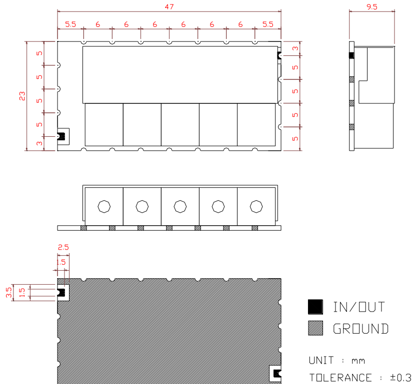
[ Mechanical 2D Drawing ]
