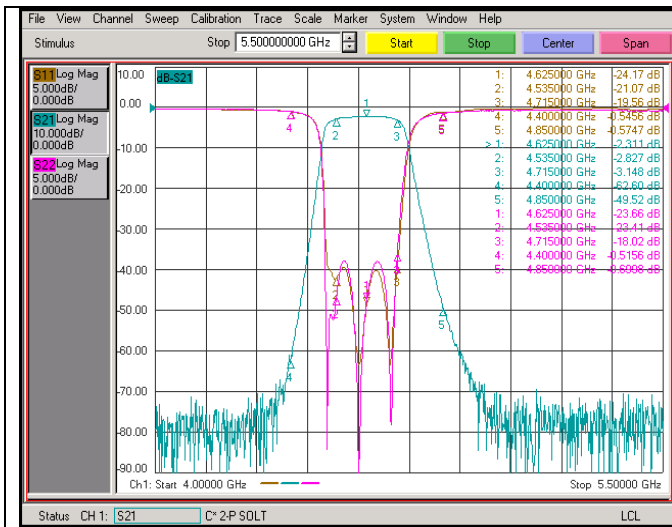
Insertion Loss, Return Loss, Rejection
