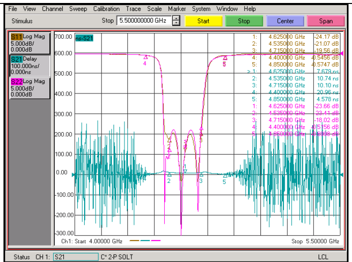
Group Delay
