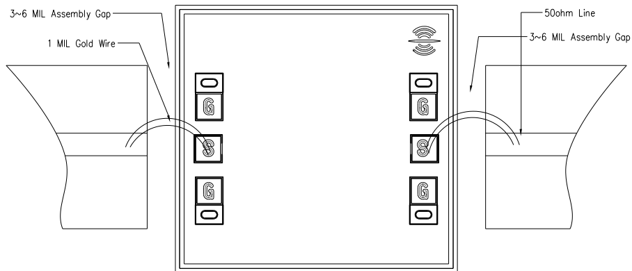
Assembly Diagram
