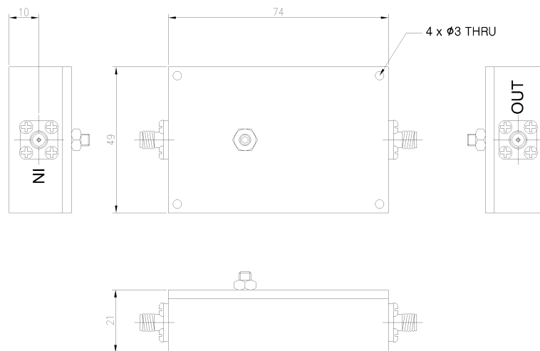
[ Mechanical 2D Drawing ]
