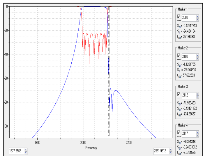
[SIMULATION CURVE]
