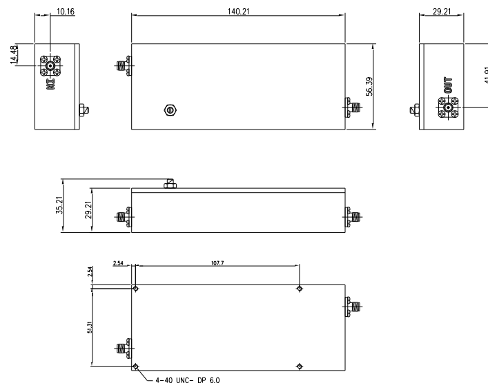
[ Mechanical 2D Drawing ]
