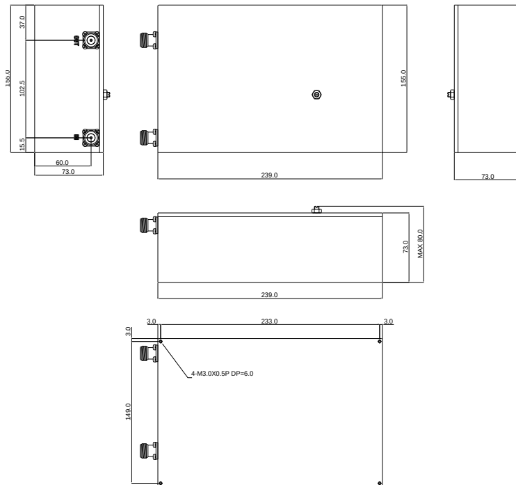
[ Mechanical 2D Drawing ]
