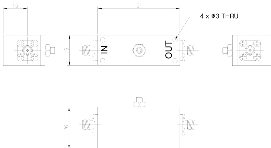
[ Mechanical 2D Drawing ]
