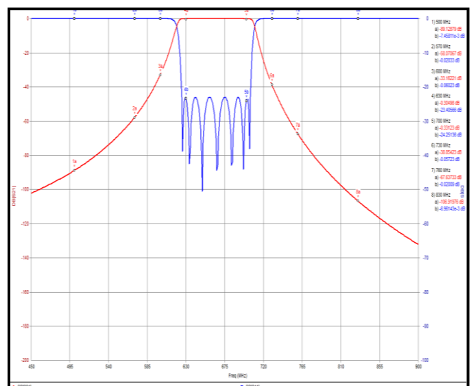
[SIMULATION CURVE]
