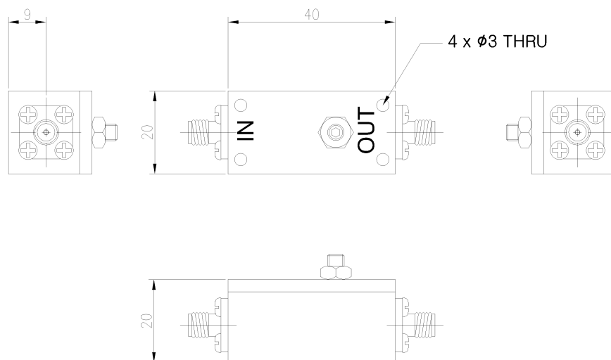
[ Mechanical 2D Drawing ]
