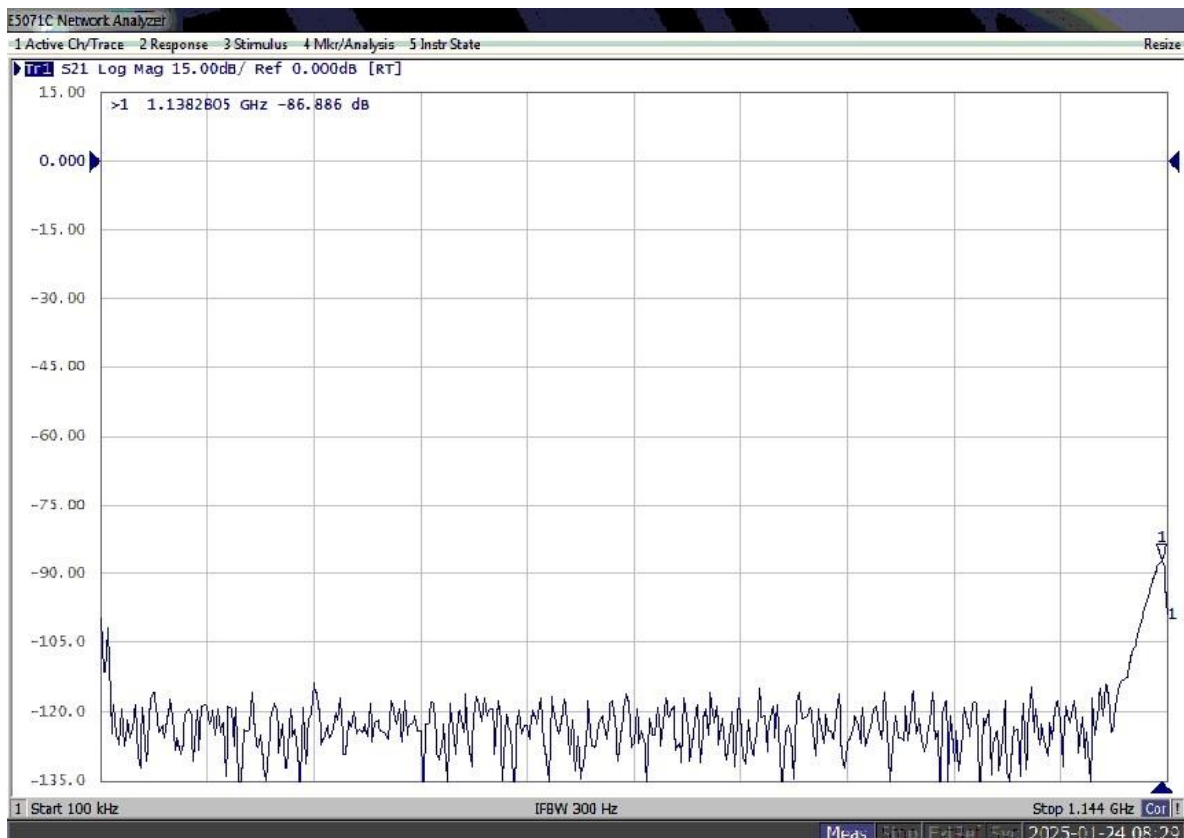
Rejection [ DC ~ 1144MHz ]
