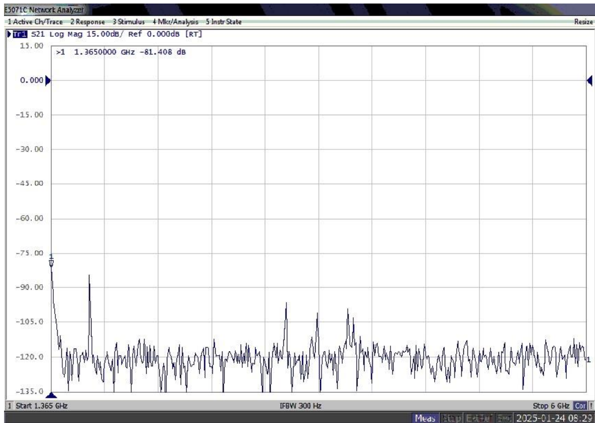
Rejection [ 1365 ~ 6000MHz ]
