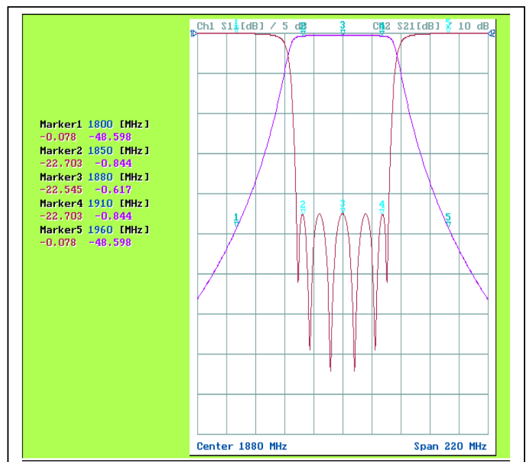
[ SIMULATION CURVE ]
