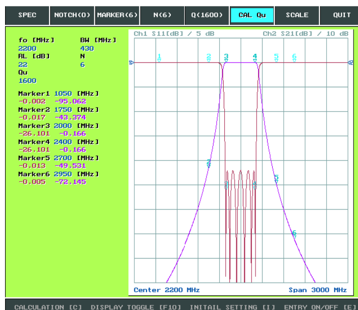
[ SIMULATION GRAPH ]
