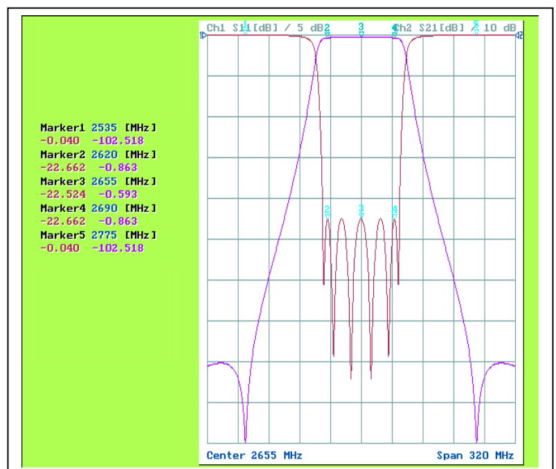
[ SIMULATION CURVE ]
