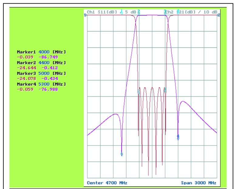
[ SIMULATION CURVE ]
