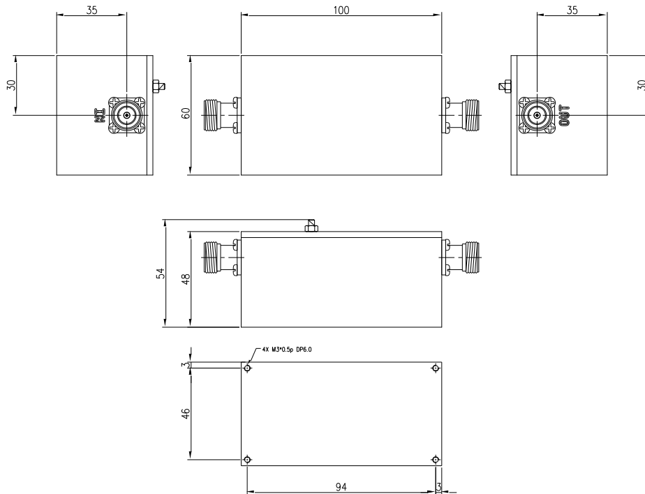
[ Mechanical 2D Drawing ]
