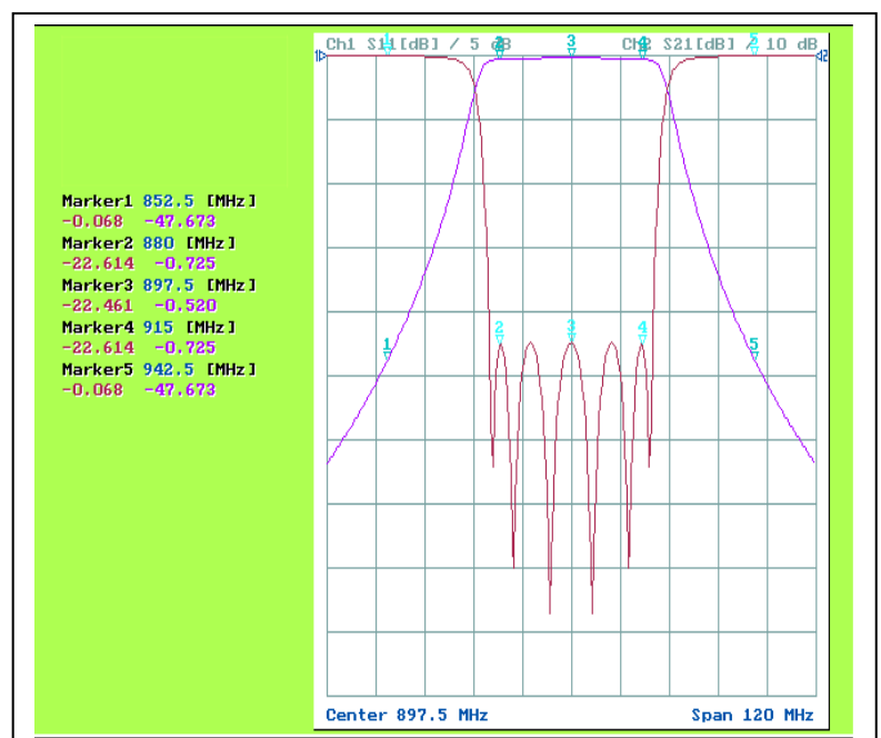
[ SIMULATION CURVE ]
