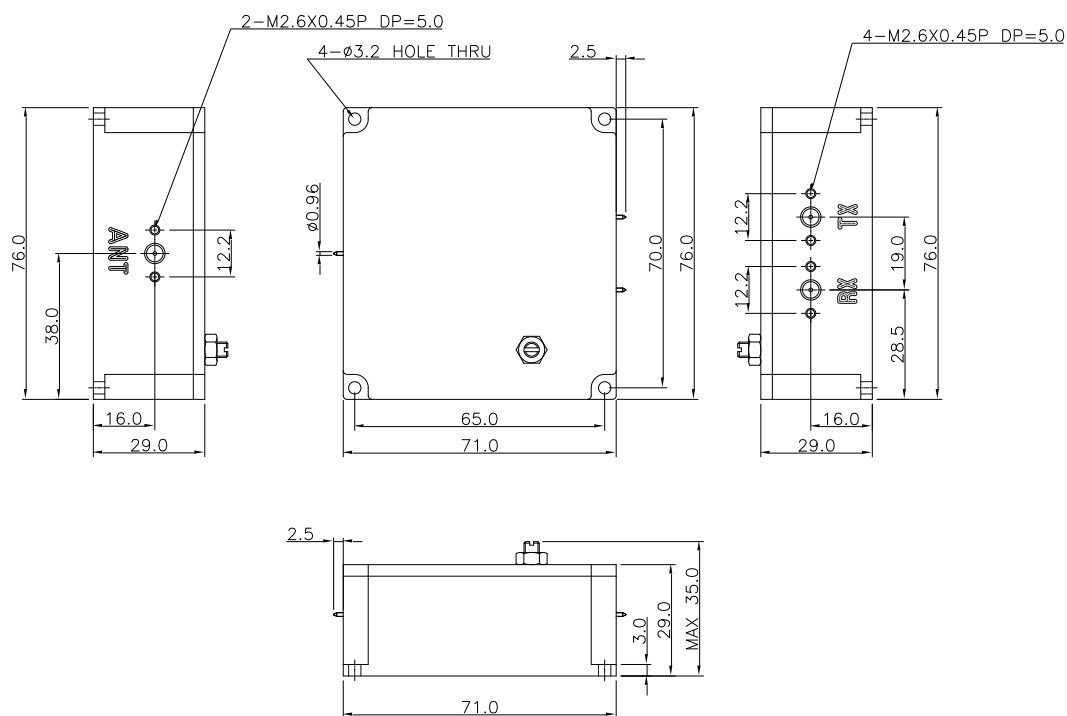
[Mechanical 2D Drawing]
