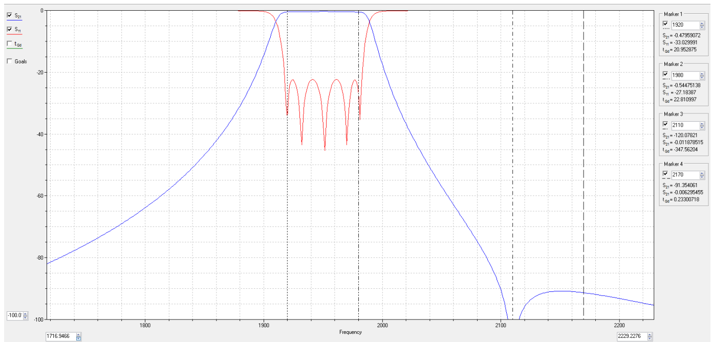
RX path
