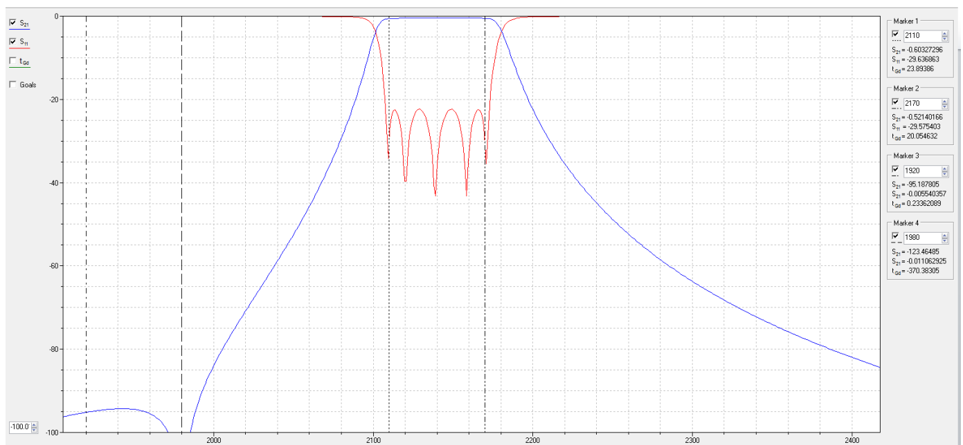
TX path
