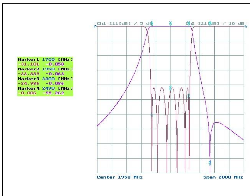
[ SIMULATION PLOT ]
