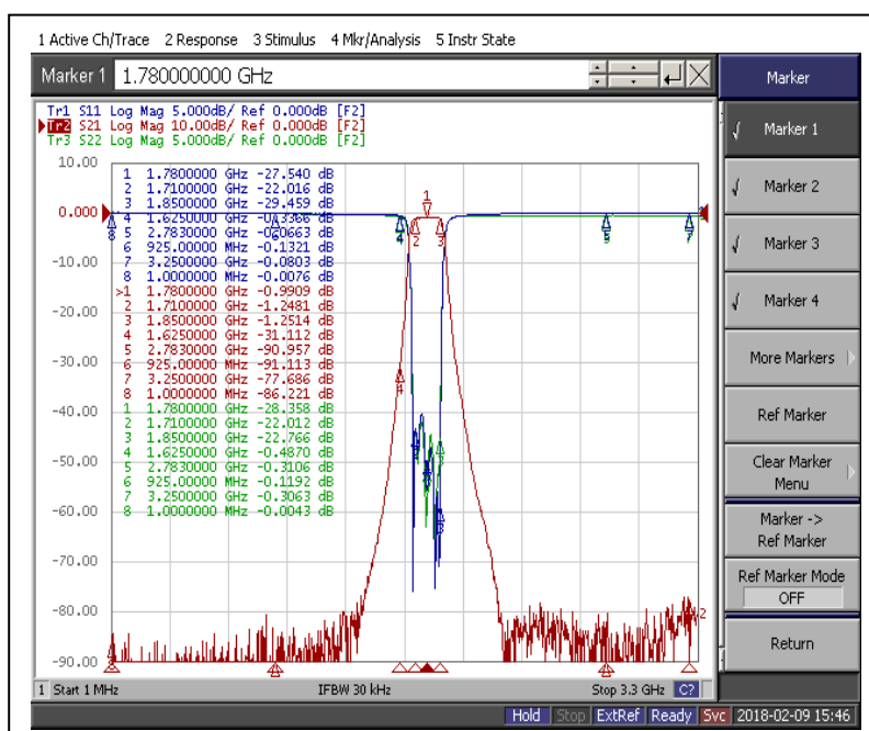
[ TEST CURVE ]
