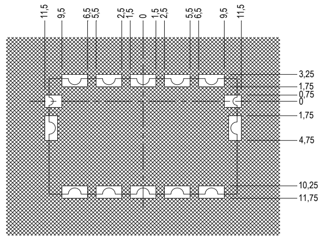
SOLDER RESISTER
