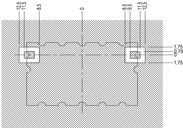
LAND PATTERN
