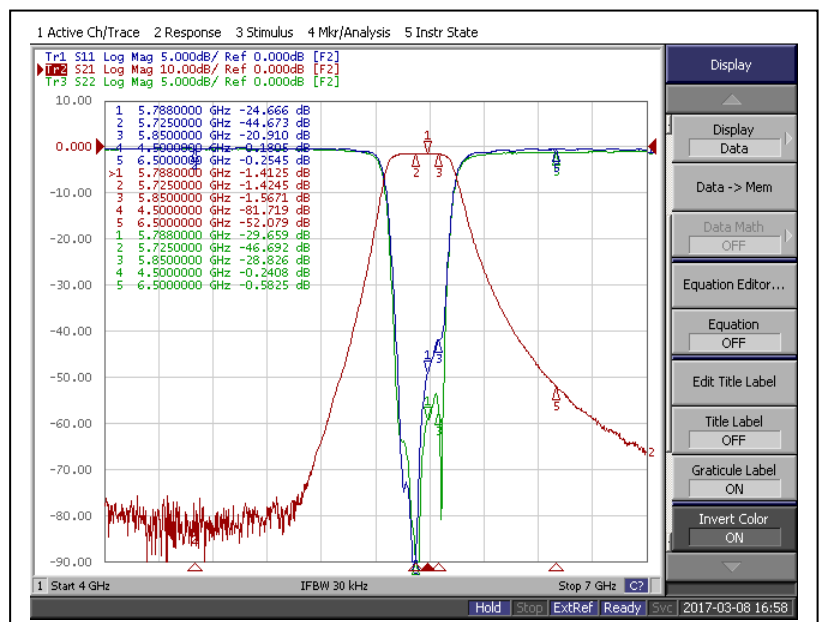
[ TEST CURVE ]
