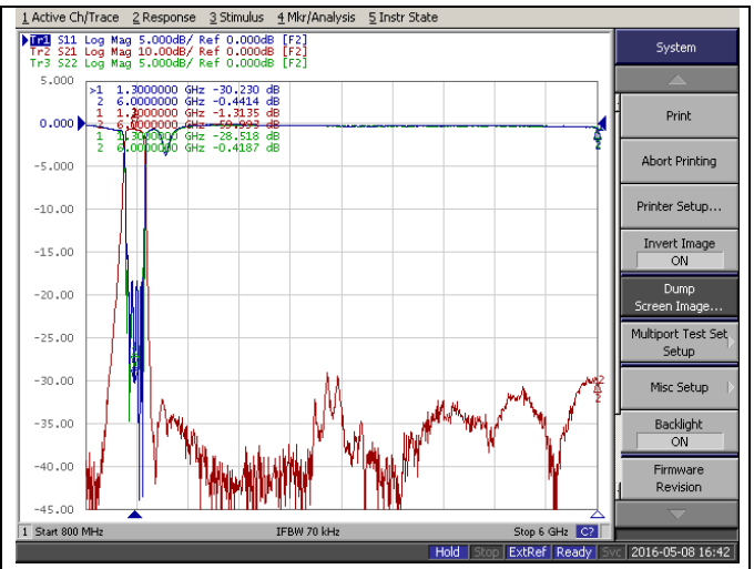
Harmonics up to 6GHz
