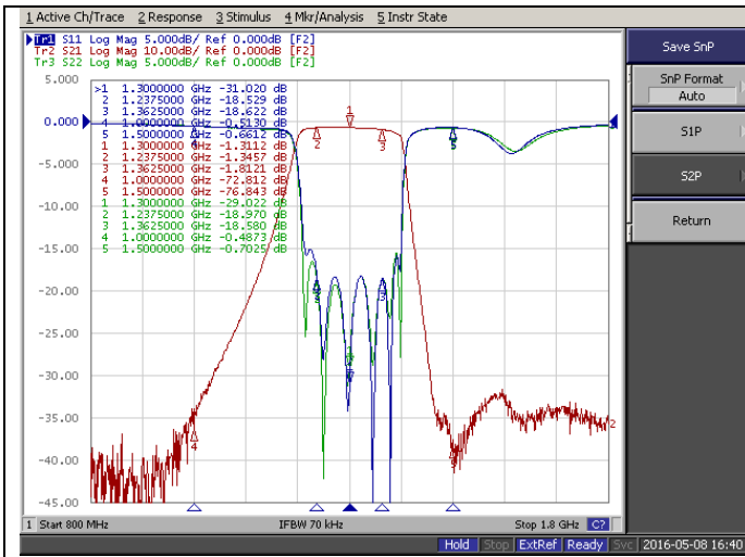
Insertion Loss, Return Loss, Attenuation
