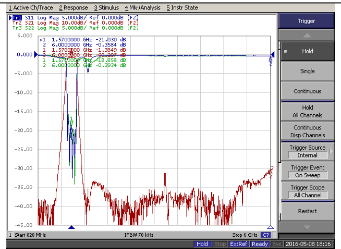
Harmonics up to 6GHz
