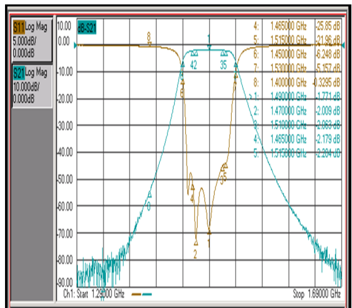
[ Test Curve ]
