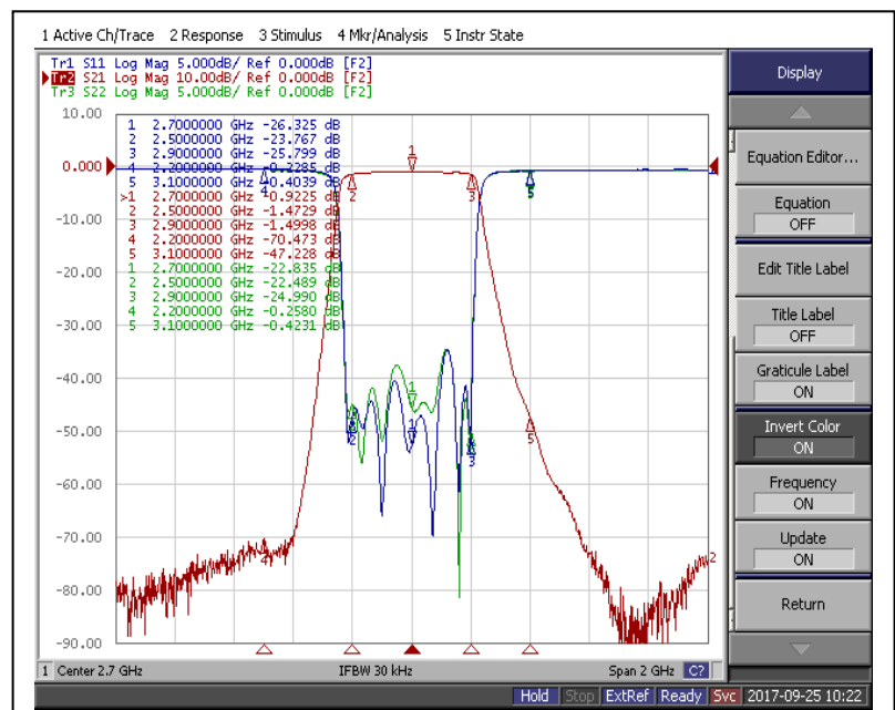
[ SIMULATION CURVE ]
