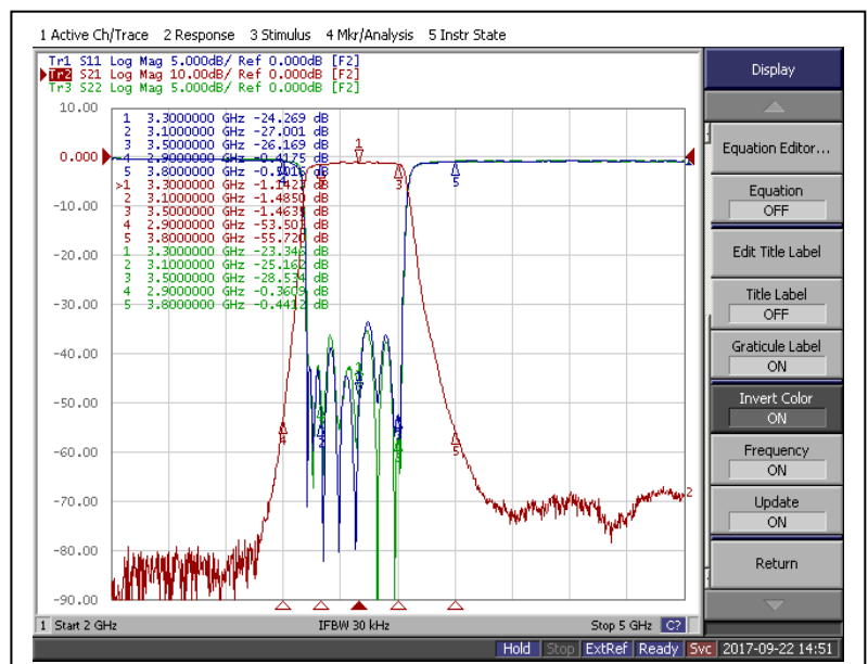
[ SIMULATION CURVE ]
