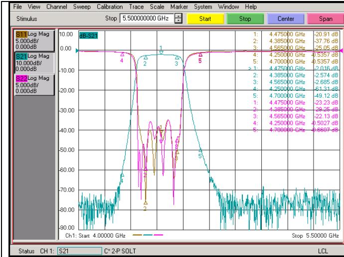
Insertion Loss, Return Loss, Rejection
