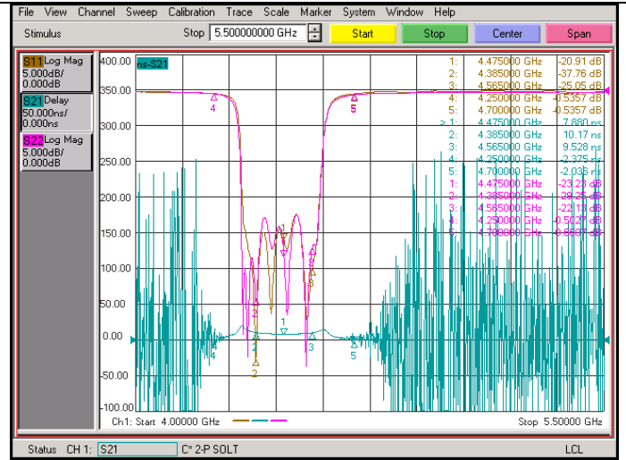
Group Delay
