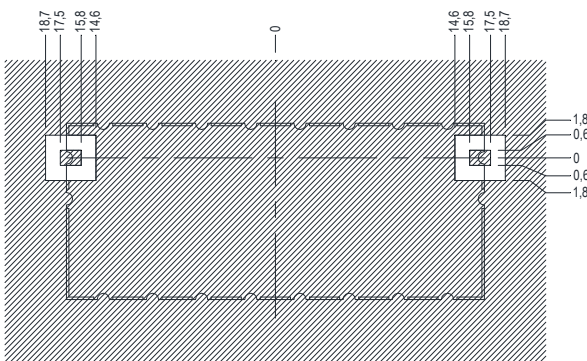
LAND PATTERN
