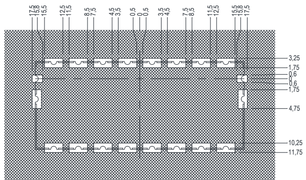
SOLDER RESISTOR
