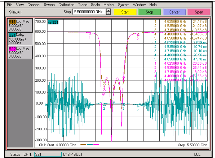
Group Delay
