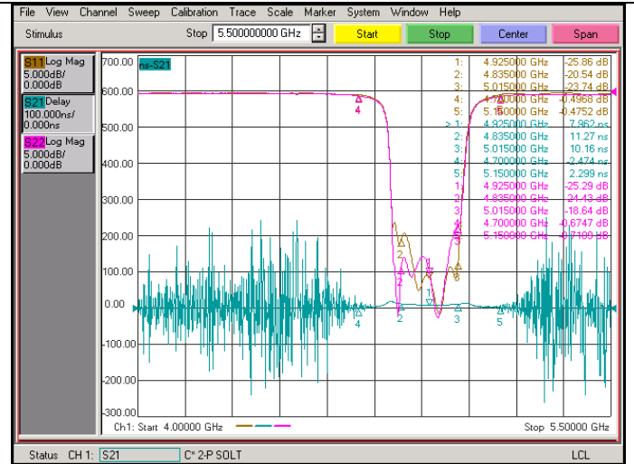
Group Delay
