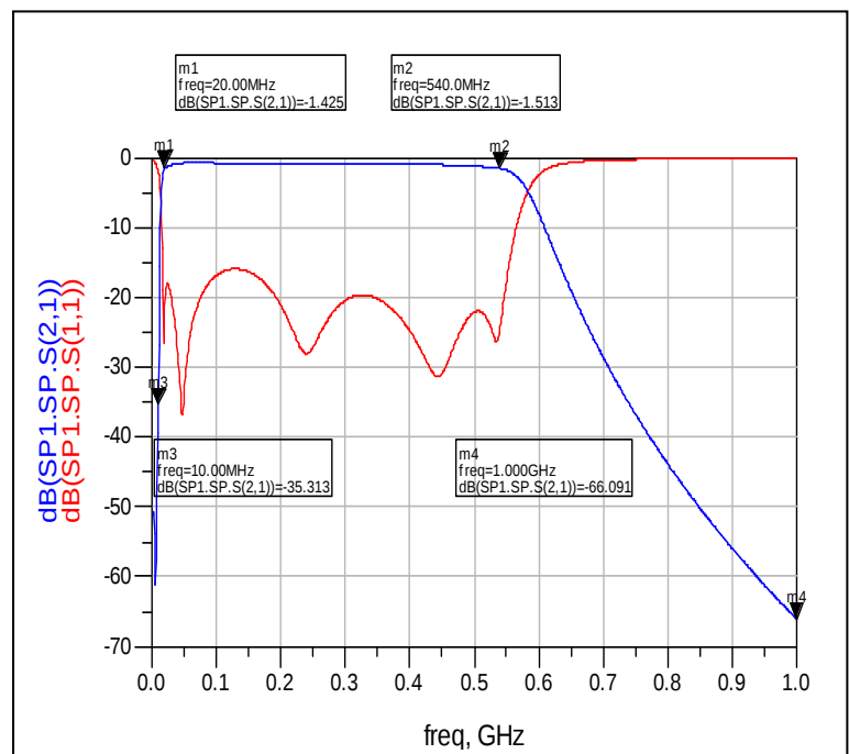
[ Simulation Curve ]
