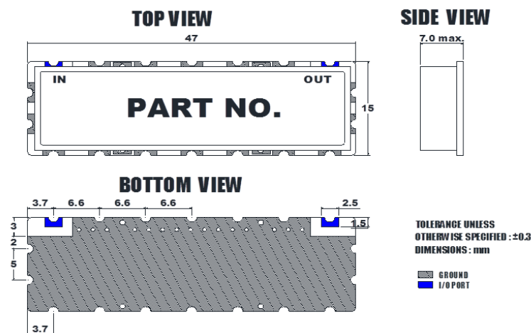
[ Mechanical 2D Drawing ]
