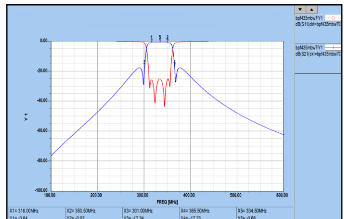
[ Simulation Curve ]
