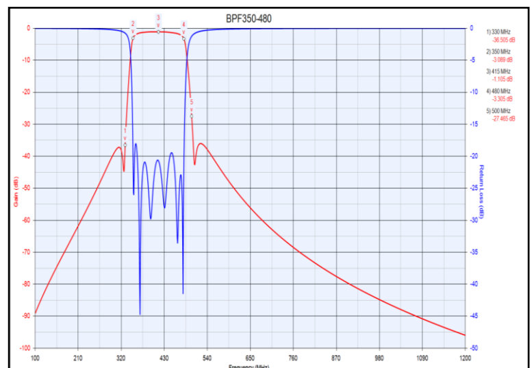
[Simulation Curve]
