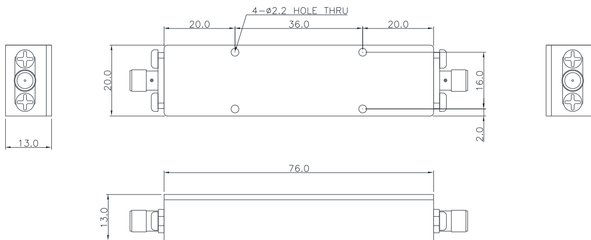
[ Mechanical 2D Drawing ]
