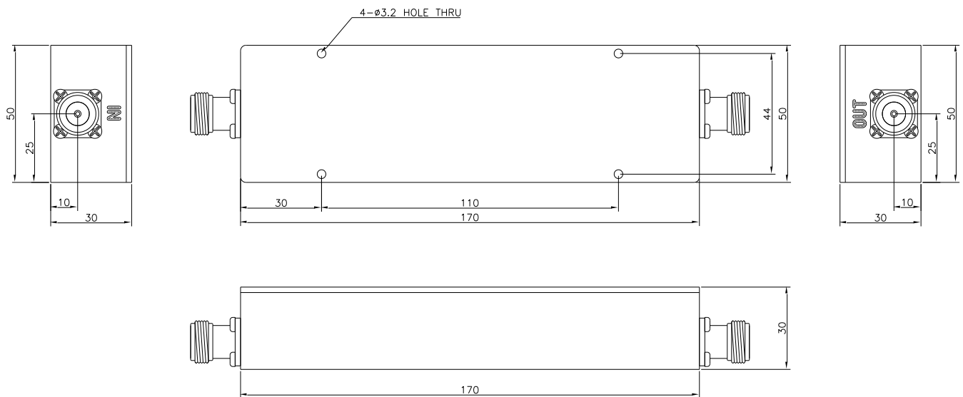
[ Mechanical 2D Drawing ]
