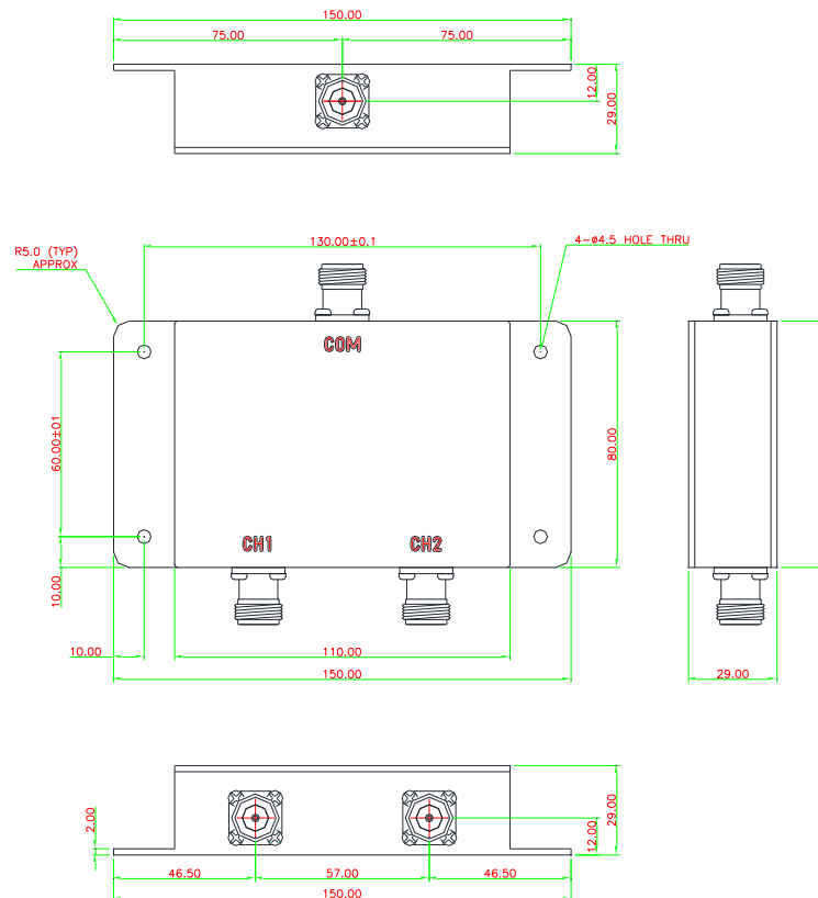
[ Mechanical 2D Drawing ]
