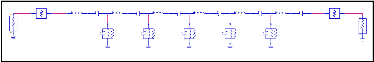
Topology: 11pole
