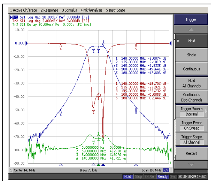
[ TEST CURVE ]
