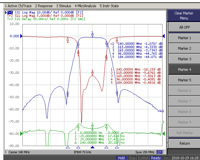
3dB Bandwidth
