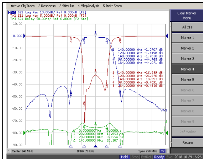
1dB Bandwidth
