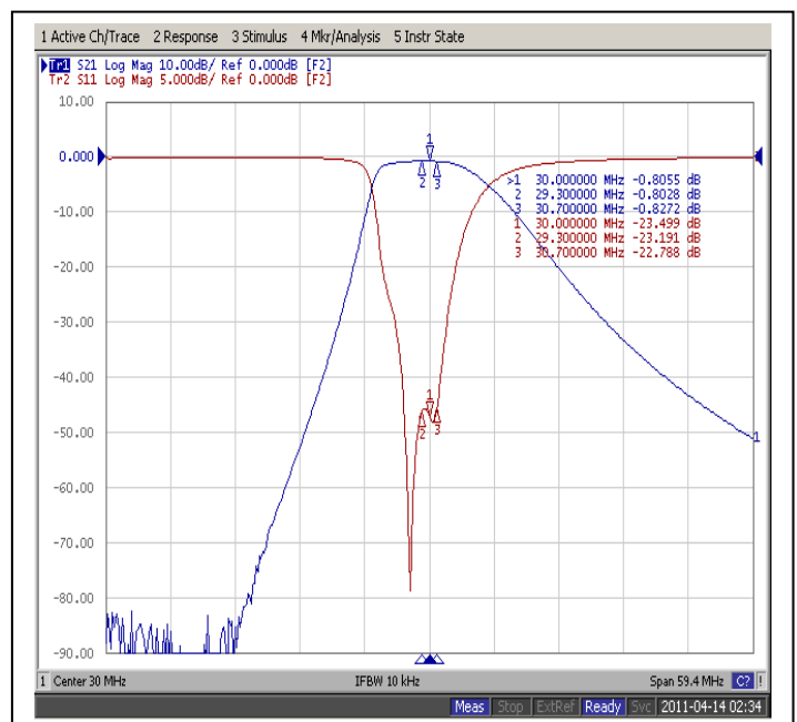
[ TEST CURVE ]
