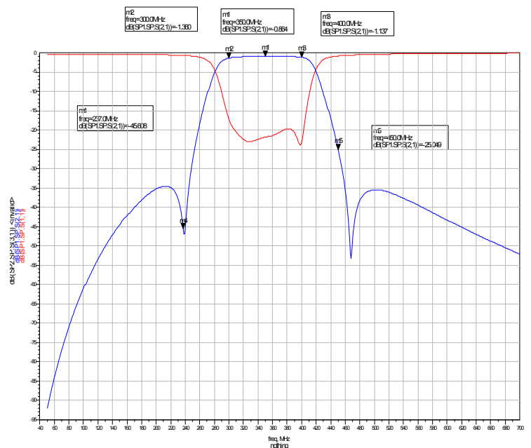
[ SIMULATION GRAPH ]
