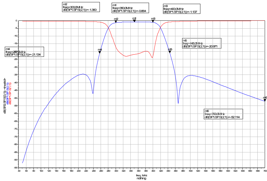
[ 20dB Bandwidth ]
