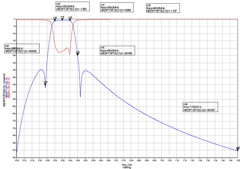
[ Rejection @ 1500MHz ]
