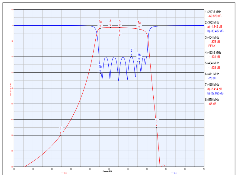
[ SIMULATION GRAPH ]
