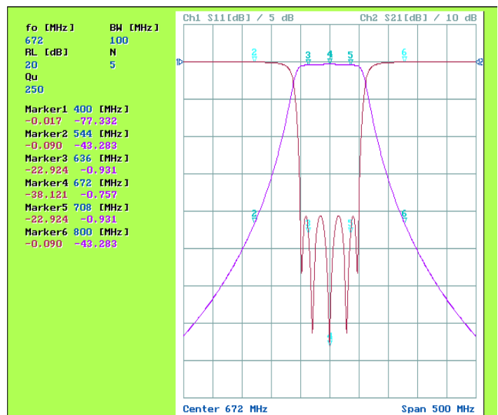
[ Simulation Graph ]
