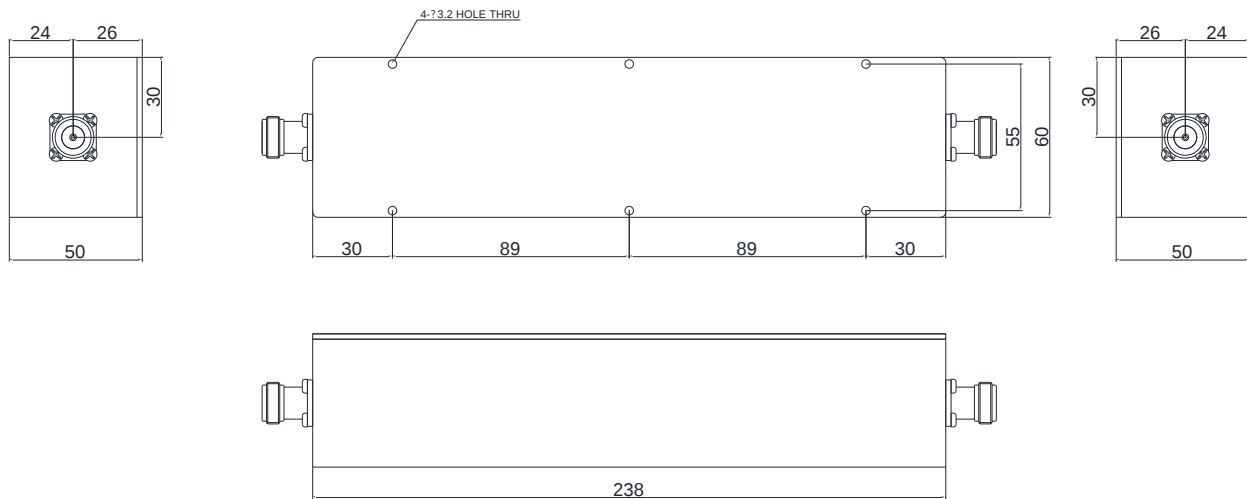
[ Mechanical 2D Drawing ]
