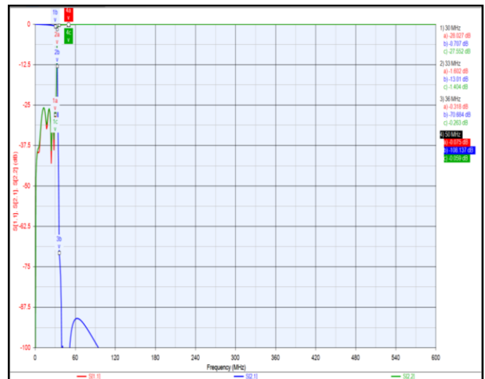
[ Simulation Curve ]
