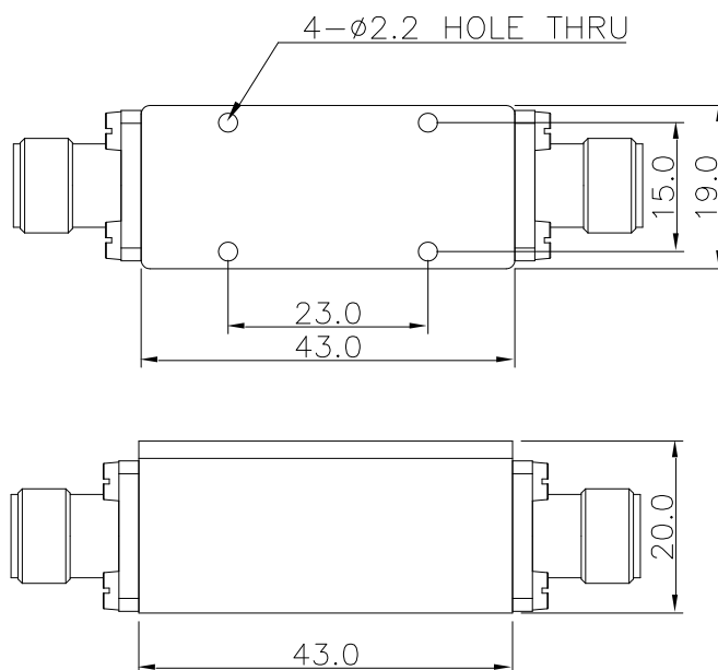
[ Mechanical 2D Drawing ]
