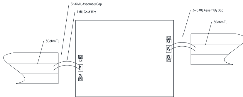
Assembly Diagram
